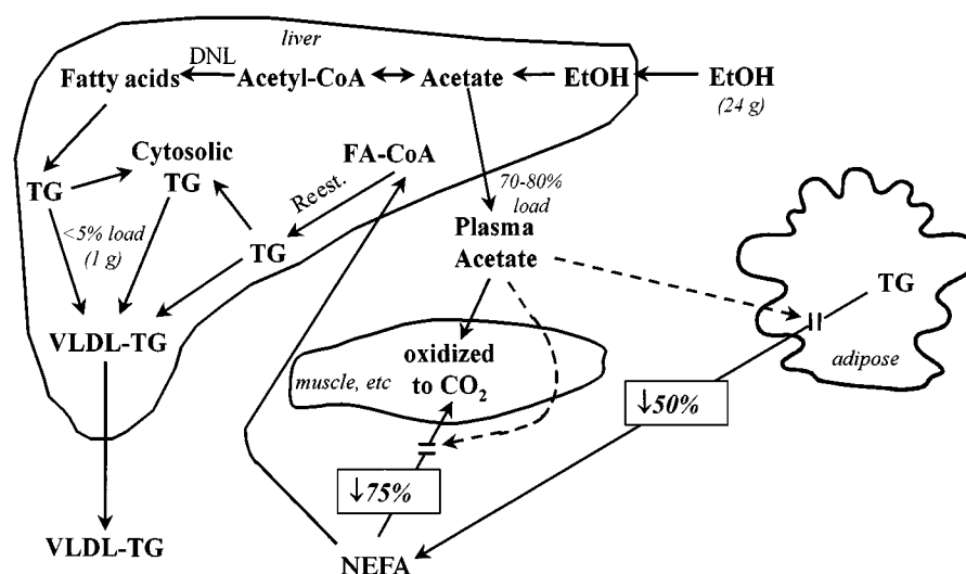
FIGURE 7. Model of whole-body lipid metabolism after consumption of moderate quantities of ethanol. See Discussion for details. EtOH, ethanol; DNL, de novo lipogenesis; TG, triacylglycerol; FA-CoA, fatty-acyl-CoA synthase; Reest, reesterification of fatty-acyl-CoA synthase to triacylglycerol; NEFA, nonesterified fatty acids.
